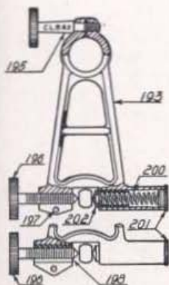
TELESCOPE CLAMP Telescope Clamp
