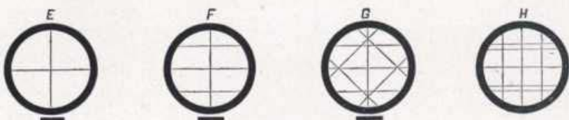
The Cross-hairs for Transits
