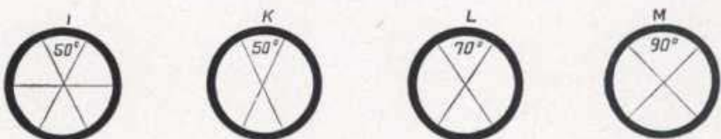
The Cross-hairs for Plain Triangulation Transits
