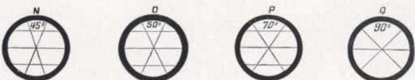
The Cross-hairs for Complete Triangulation Theodolites (N, O and P arranged for stadia work)
