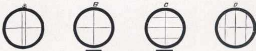
The Cross-hair Arrangements for Dumpy and Wye Levels (Diaphragms C and D are provided with Stadia hairs)
